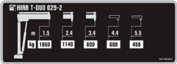
Capacity plate HIAB T-DUO 029-2
