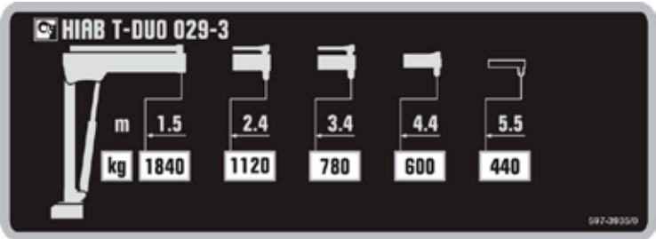
Capacity plate HIAB T-DUO 029-3
