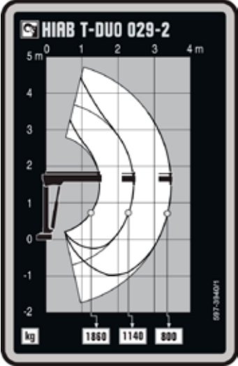
Load diagram HIAB T-DUO 029-2
