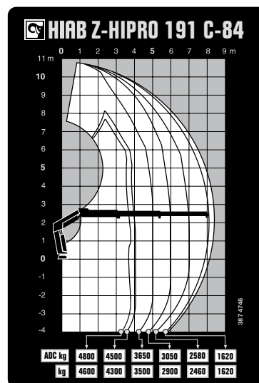
Load diagram HIAB Z-HIPRO 191
